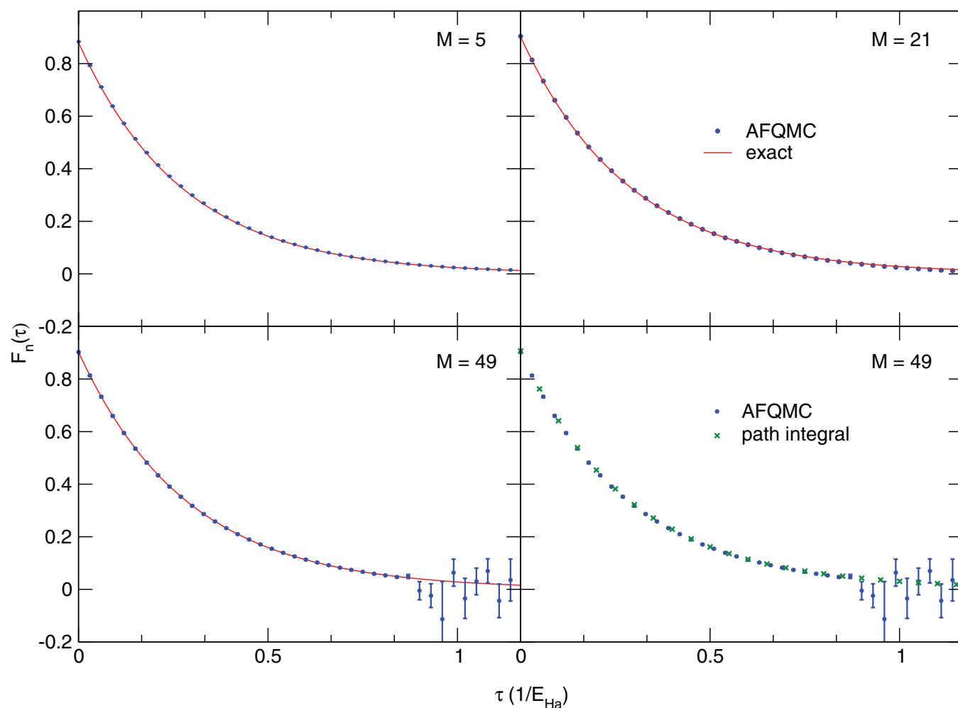
FIG. 4. Imaginary time correlation function of the momentum shift operator relative to M = 5, 21, 49 at r_s = 1 for N_\uparrow = 1, N_\downarrow = 1 . In the right lower box, comparison between AFQMC and exact Path Integral QMC calculations is given. When not visible, error bars are smaller than the symbol size.
