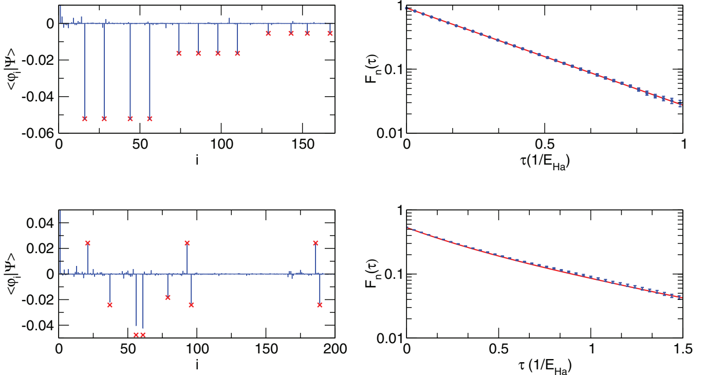
FIG. 3. Left column: exact nonvanishing (red crosses) and reconstructed (blue columns) components of the ground state for systems with N_\uparrow, N_\downarrow = (1, 1) , (5, 0) (top to bottom), relative to all elements of the basis except |\phi_1\rangle = |\Psi_T\rangle . Exact and reconstructed values of \langle \phi_1 | \Psi \rangle are, respectively, 0.9937, 0.9939(2) and 0.9926, 0.9885(3). Right column: exact (red line) and reconstructed (circles) imaginary time correlation function of the density fluctuation operator with \mathbf{n} = (1, 0) for systems with N_\uparrow, N_\downarrow = (1, 1) , (5, 0) (top to bottom). When not visible, error bars are smaller than the symbol size.
